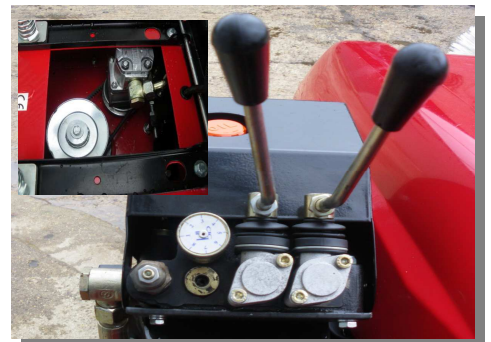
FKDR/HydrDL includes hydraulic lift — lower - angling and variable brush speed. The on board oil pump is mounted under the seat.
